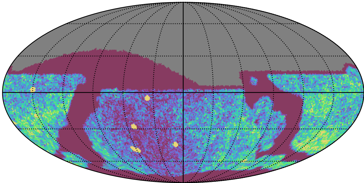
too_5_1v3.4_10yrs Yr 1 all bands: NVisits
