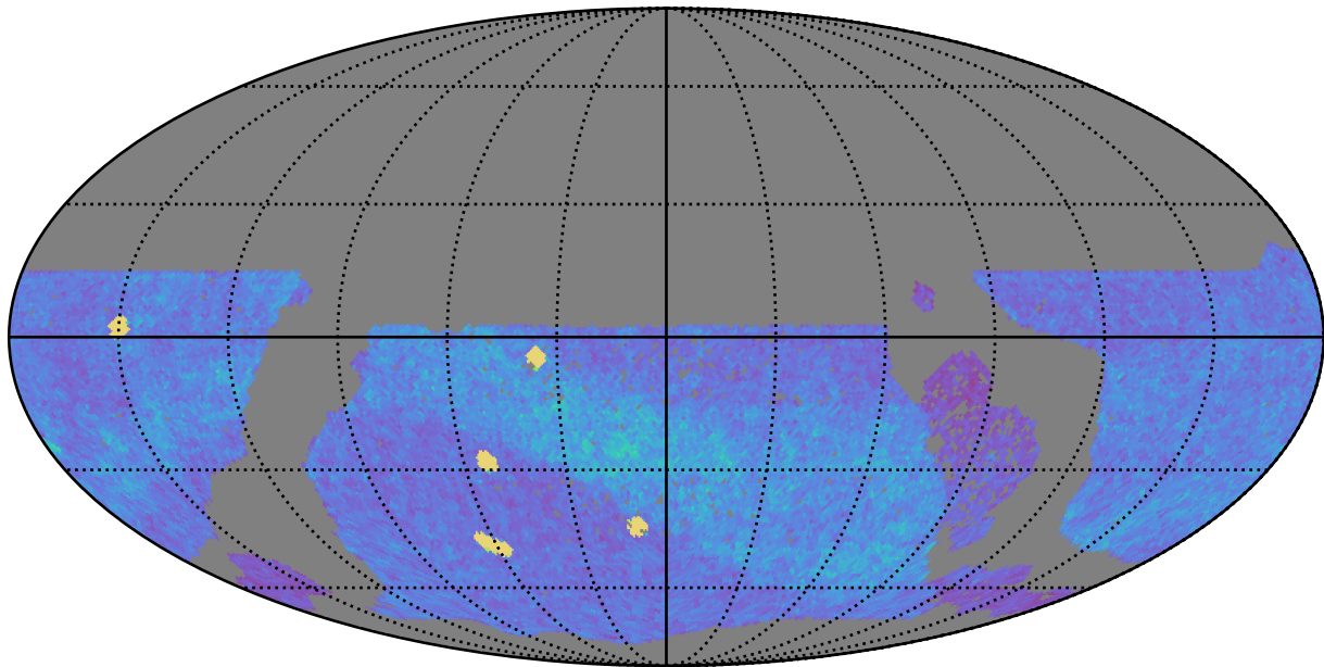
too_5_1v3.4_10yrs WFD z band: NVisits
