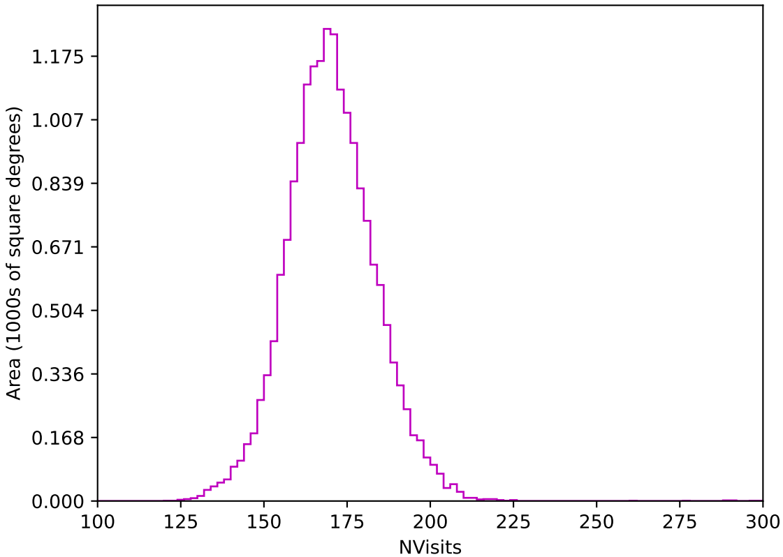
too_5_1v3.4_10yrs WFD z band: NVisits
