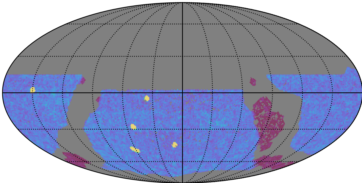
too_5_1v3.4_10yrs WFD y band: NVisits
