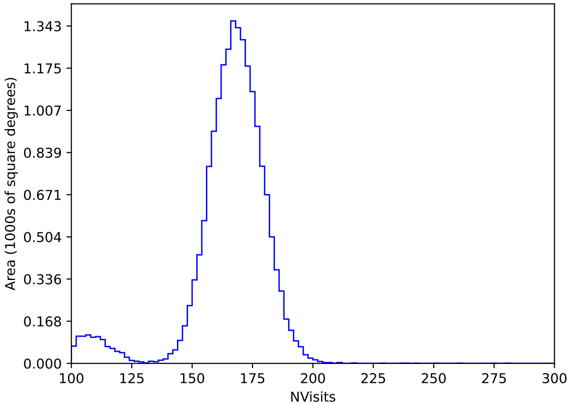
too_5_1v3.4_10yrs WFD y band: NVisits
