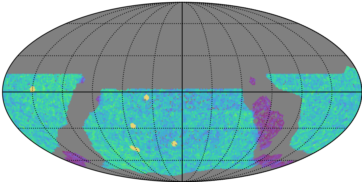
too_5_1v3.4_10yrs WFD u band: NVisits
