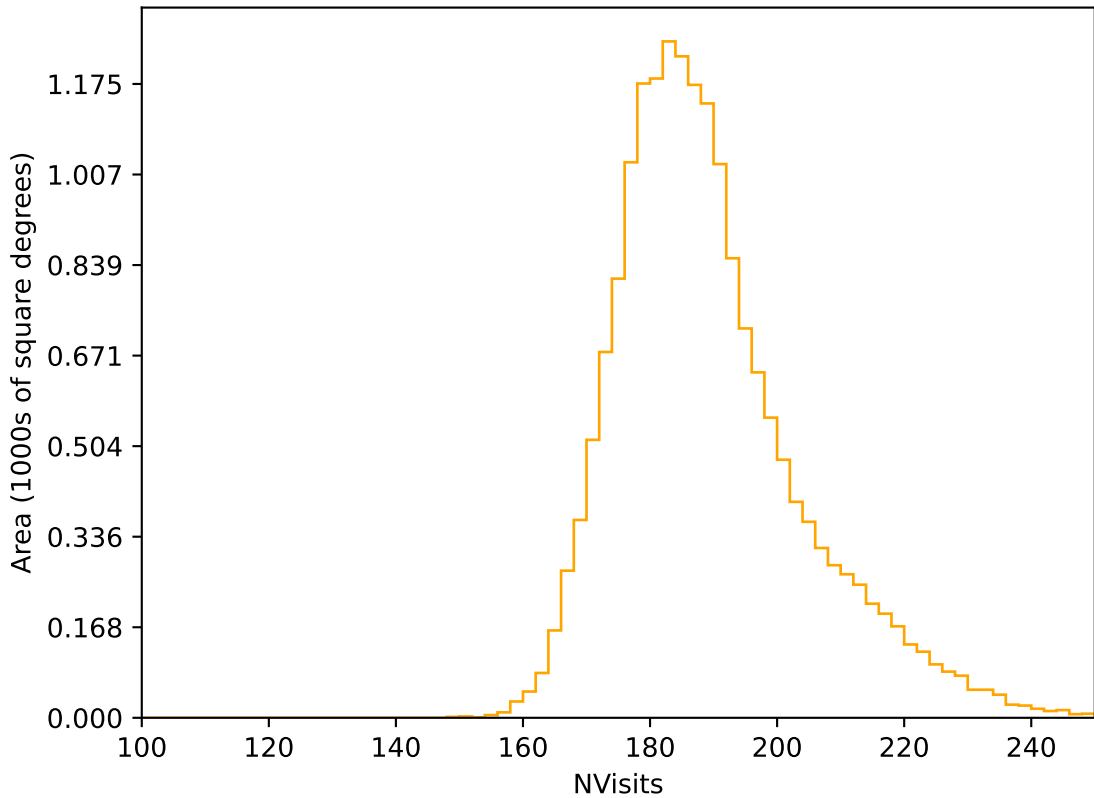
too_5_1v3.4_10yrs WFD r band: NVisits
