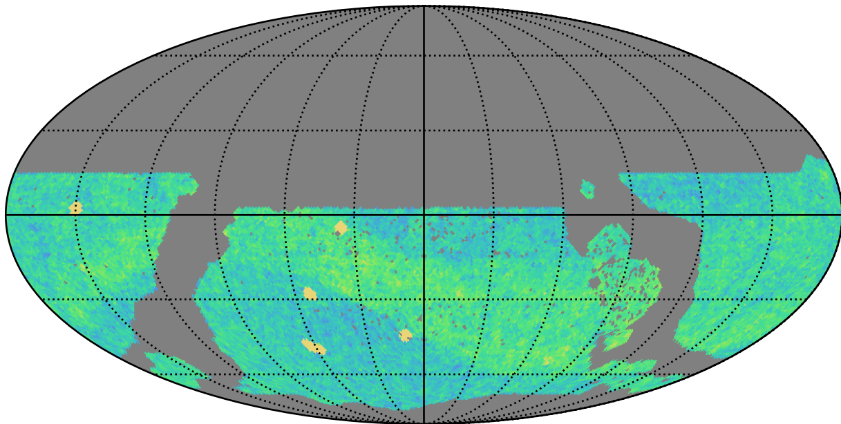
too_5_1v3.4_10yrs WFD i band: NVisits
