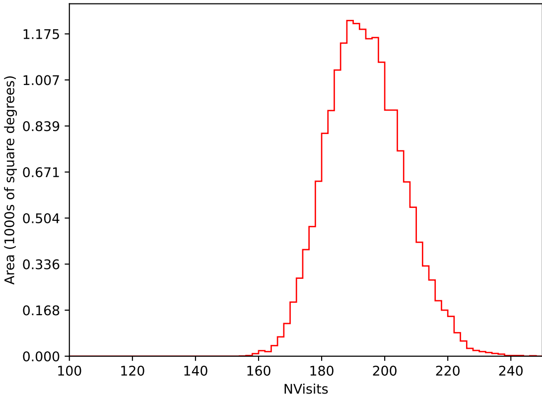
too_5_1v3.4_10yrs WFD i band: NVisits
