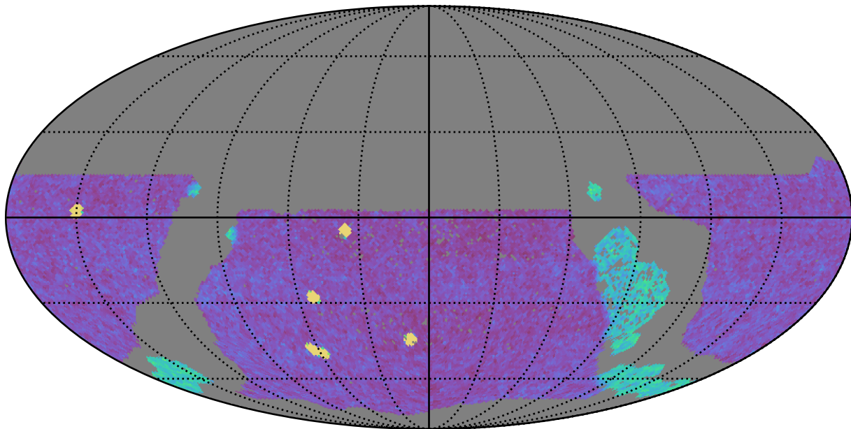
too_5_1v3.4_10yrs WFD g band: NVisits
