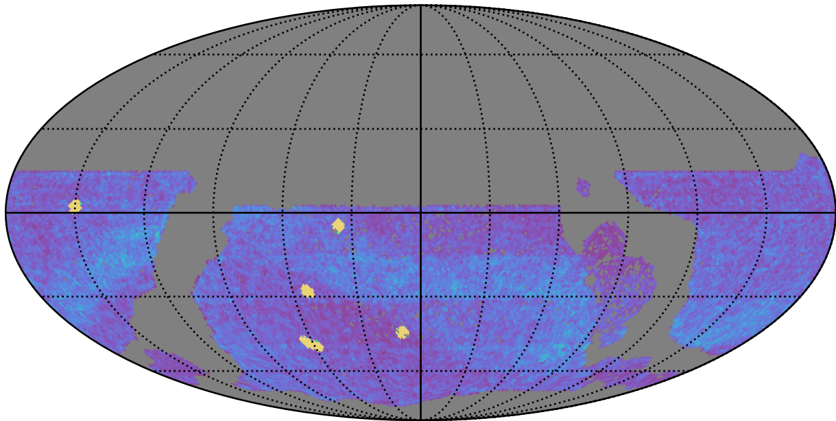
too_5_1v3.4_10yrs WFD all bands: NVisits
