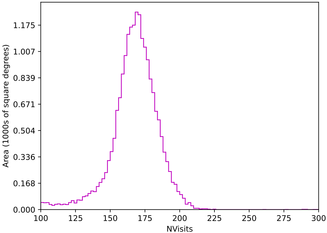
too_5_1v3.4_10yrs All sky z band: NVisits
