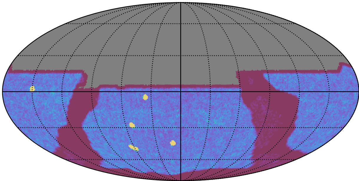
too_5_1v3.4_10yrs All sky y band: NVisits
