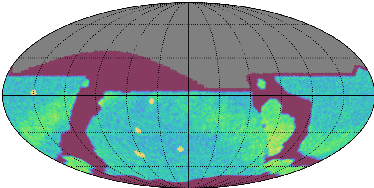
too_5_1v3.4_10yrs All sky r band: NVisits
