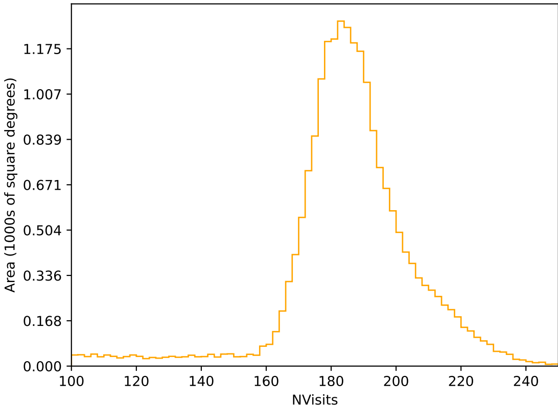
too_5_1v3.4_10yrs All sky r band: NVisits
