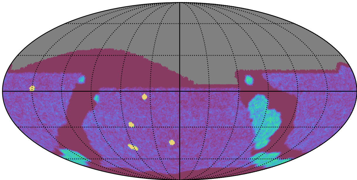
too_5_1v3.4_10yrs All sky g band: NVisits
