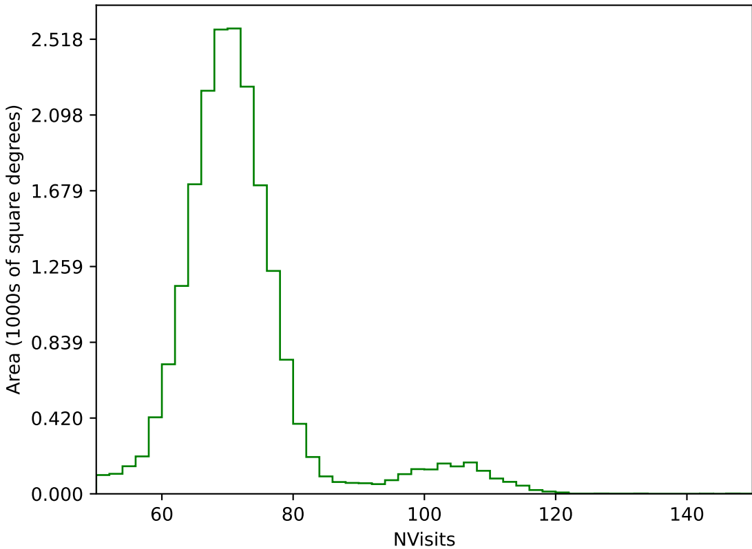
too_5_1v3.4_10yrs All sky g band: NVisits
