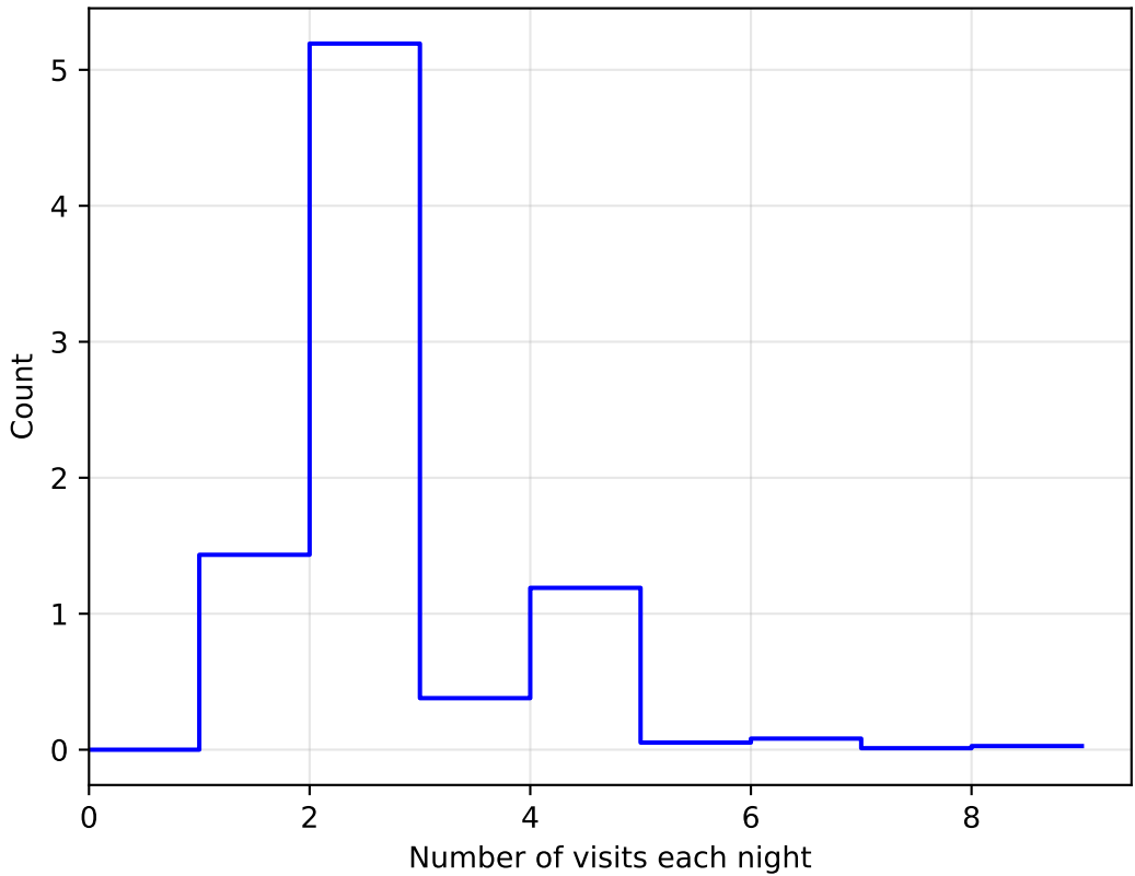
too_5_1v3.4_10yrs WFD: NVisitsPerNight
