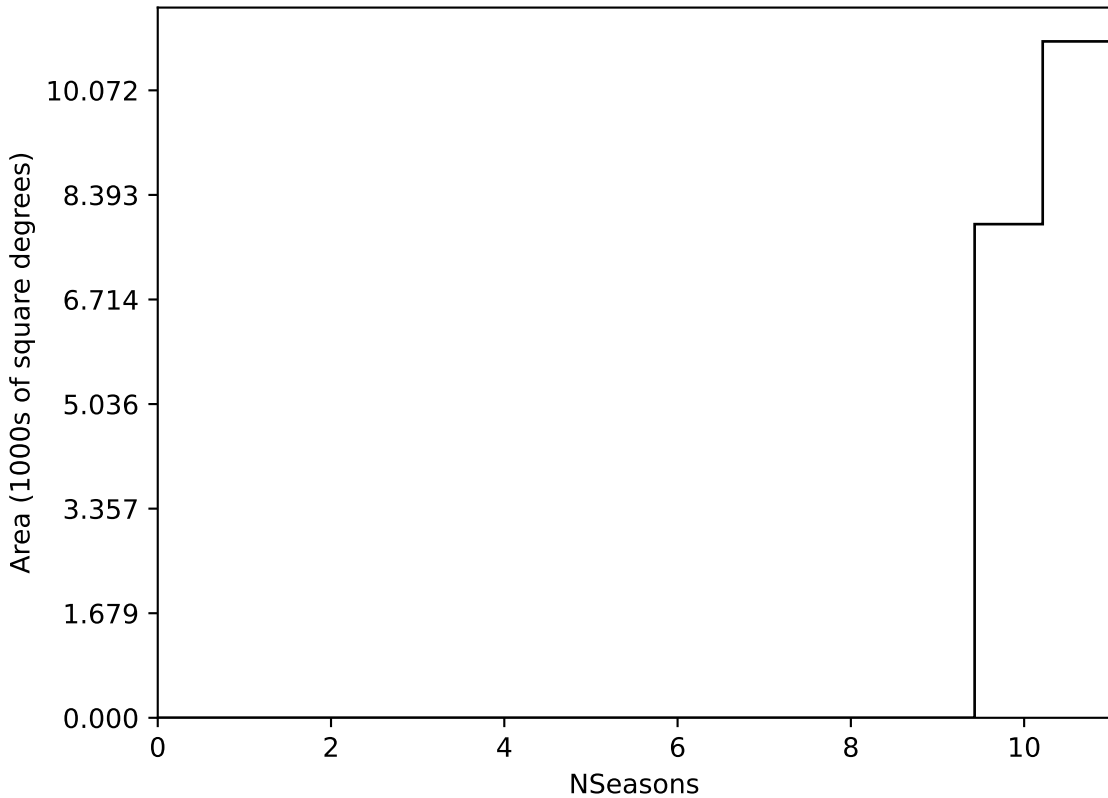
too_5_1v3.4_10yrs WFD all bands: NSeasons
