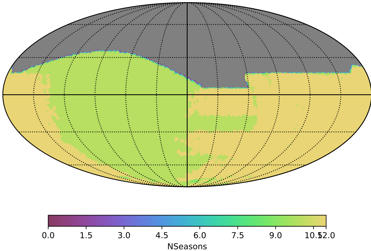
too_5_1v3.4_10yrs All sky all bands: NSeasons
