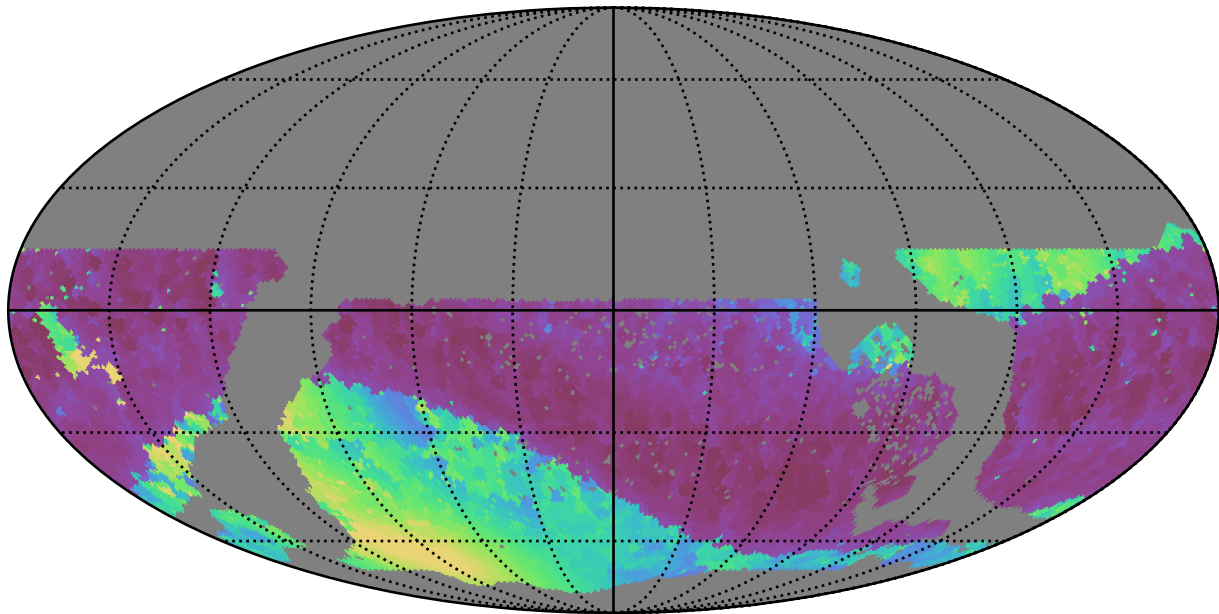
too_5_1v3.4_10yrs WFD z band: Min solarElong
