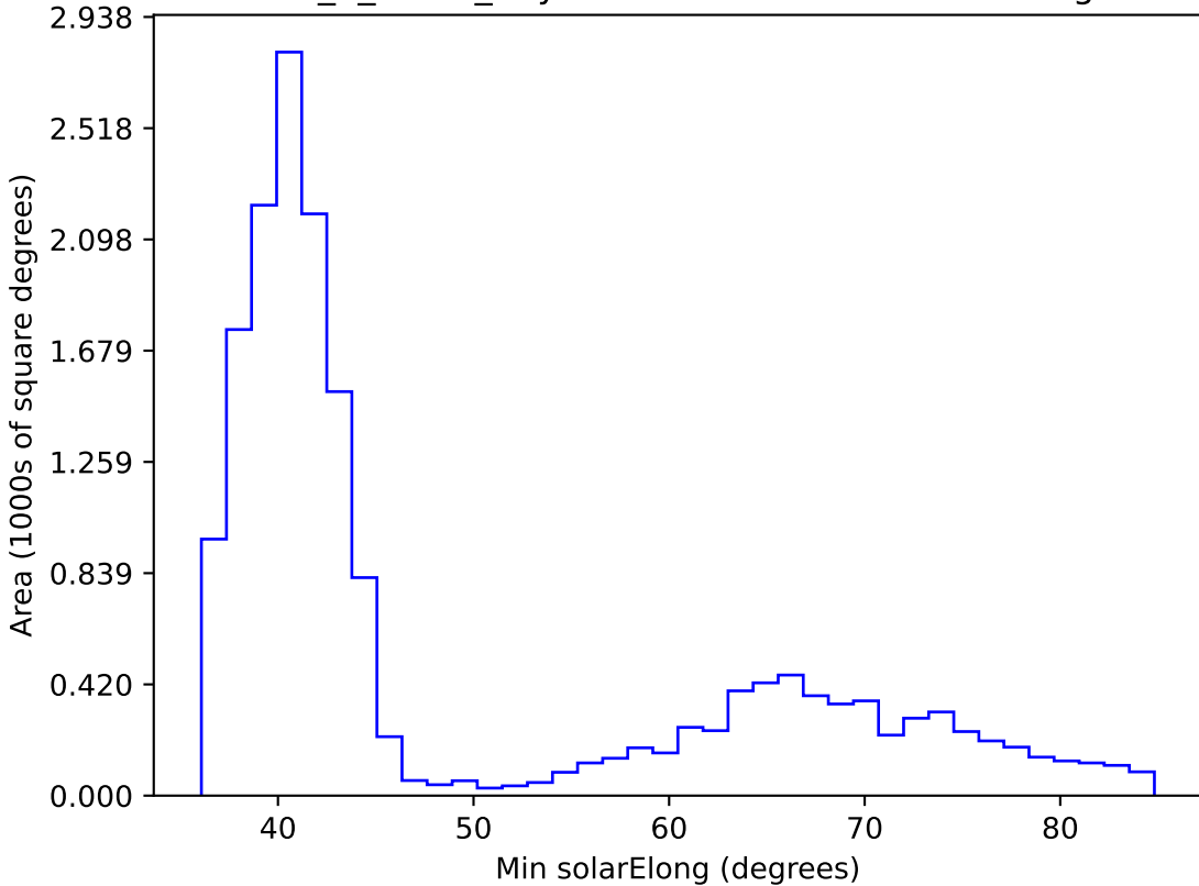
too_5_1v3.4_10yrs WFD z band: Min solarElong
