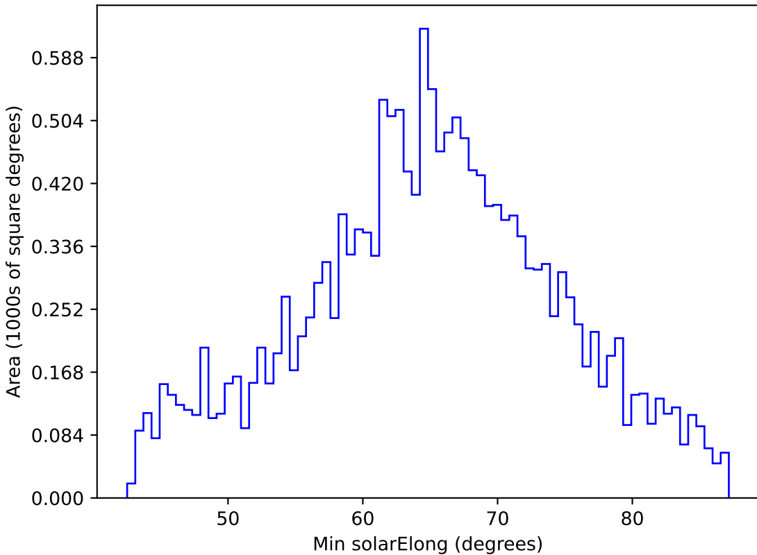
too_5_1v3.4_10yrs WFD y band: Min solarElong
