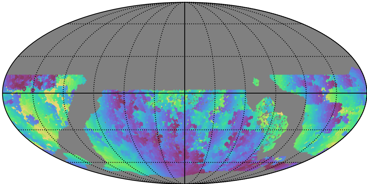
too_5_1v3.4_10yrs WFD u band: Min solarElong
