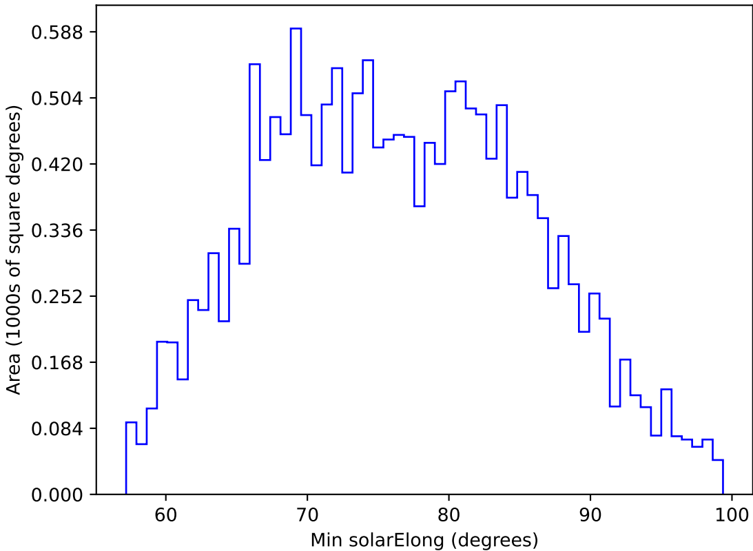
too_5_1v3.4_10yrs WFD u band: Min solarElong
