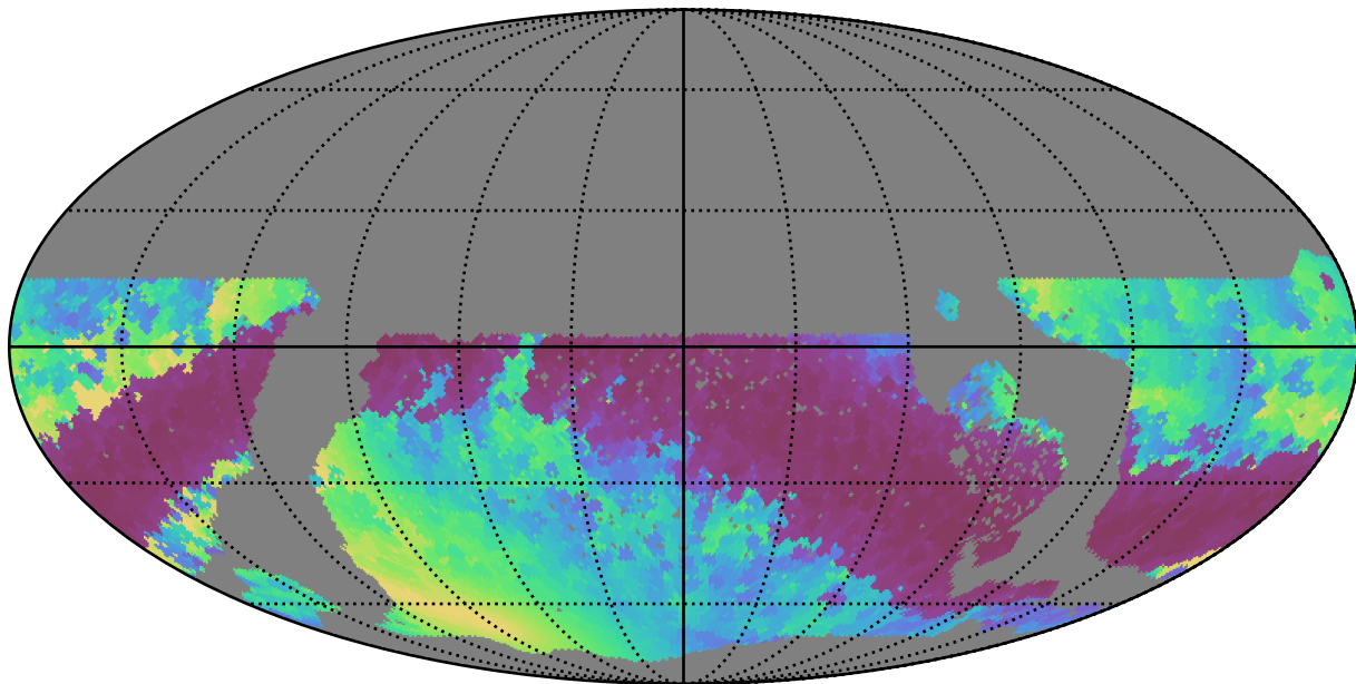
too_5_1v3.4_10yrs WFD r band: Min solarElong
