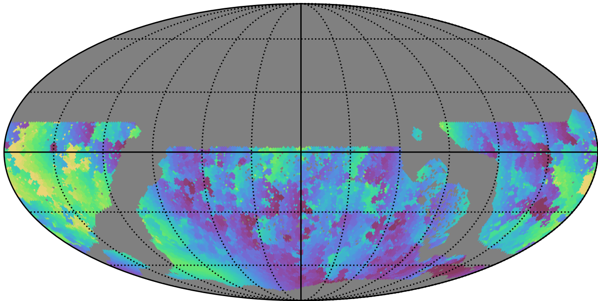
too_5_1v3.4_10yrs WFD g band: Min solarElong
