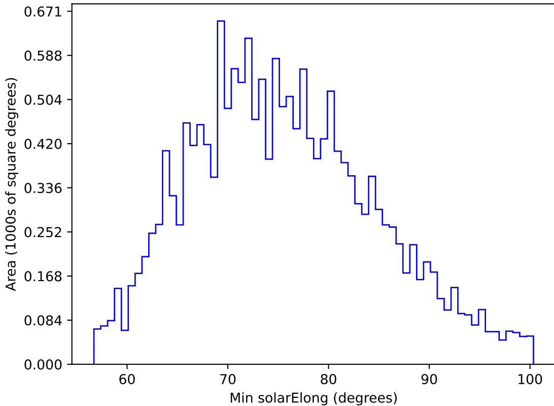
too_5_1v3.4_10yrs WFD g band: Min solarElong
