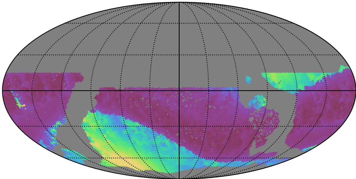
too_5_1v3.4_10yrs WFD all bands: Min solarElong
