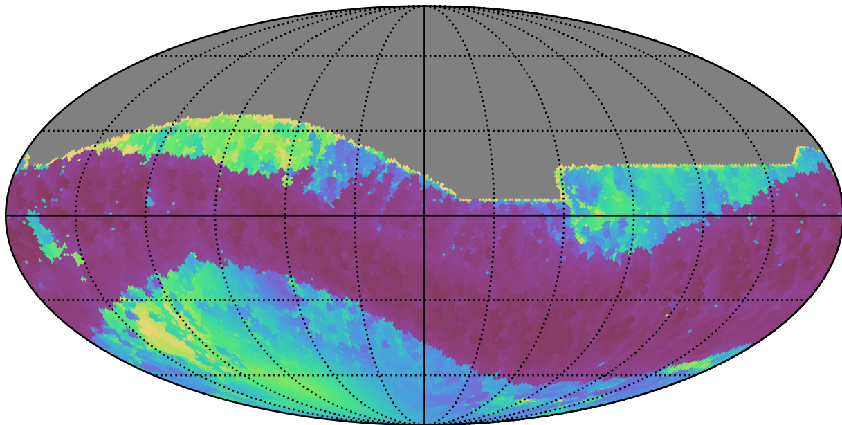
too_5_1v3.4_10yrs All sky z band: Min solarElong
