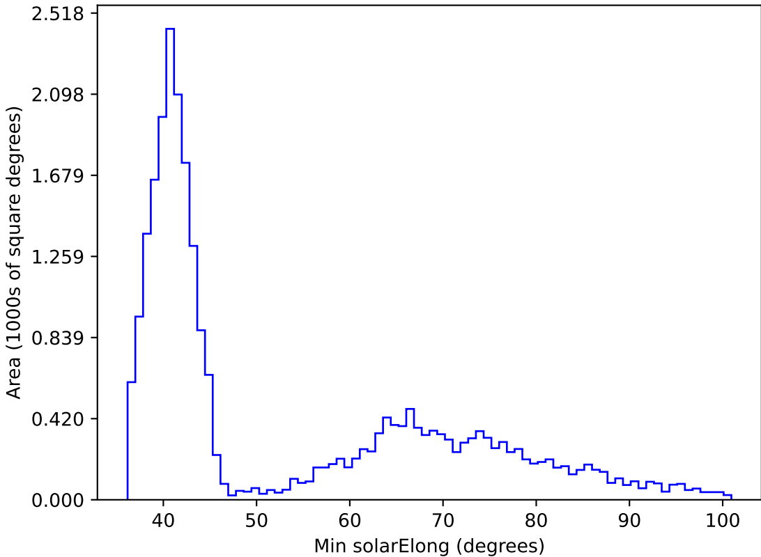
too_5_1v3.4_10yrs All sky z band: Min solarElong
