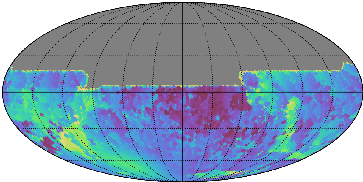
too_5_1v3.4_10yrs All sky y band: Min solarElong
