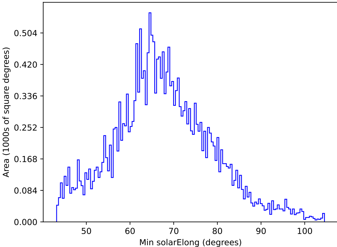
too_5_1v3.4_10yrs All sky y band: Min solarElong
