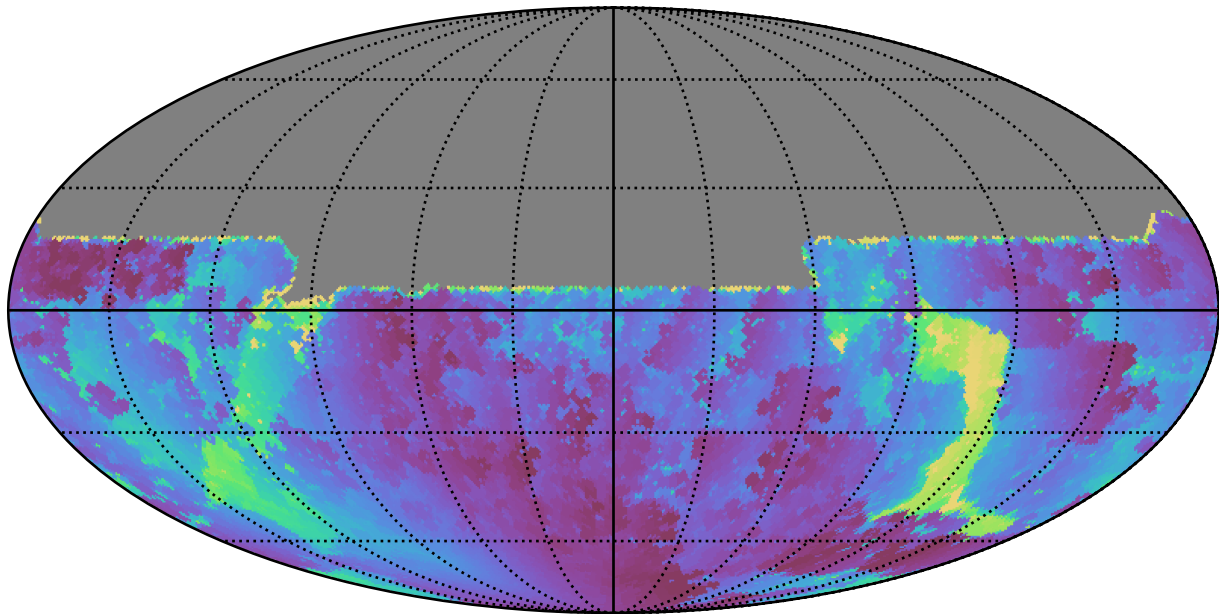
too_5_1v3.4_10yrs All sky u band: Min solarElong
