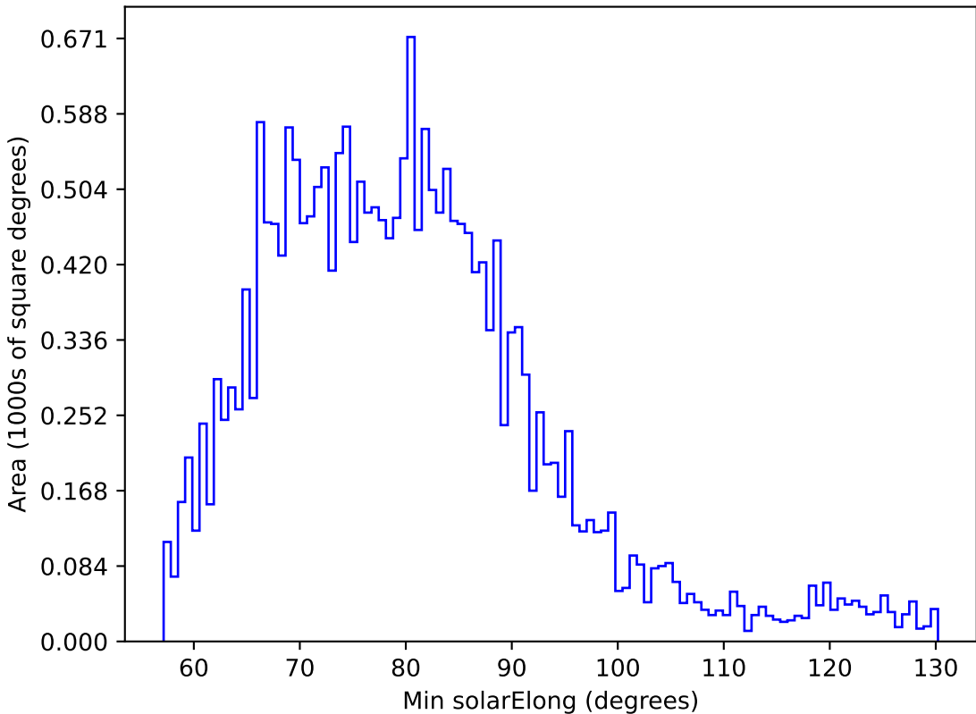
too_5_1v3.4_10yrs All sky u band: Min solarElong
