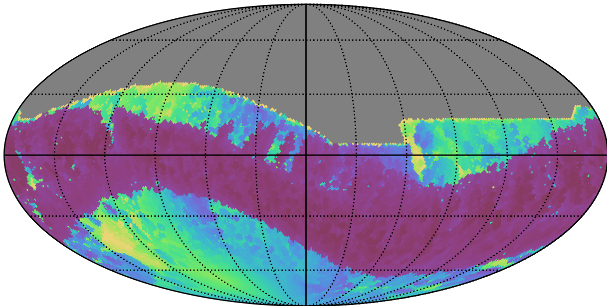
too_5_1v3.4_10yrs All sky i band: Min solarElong
