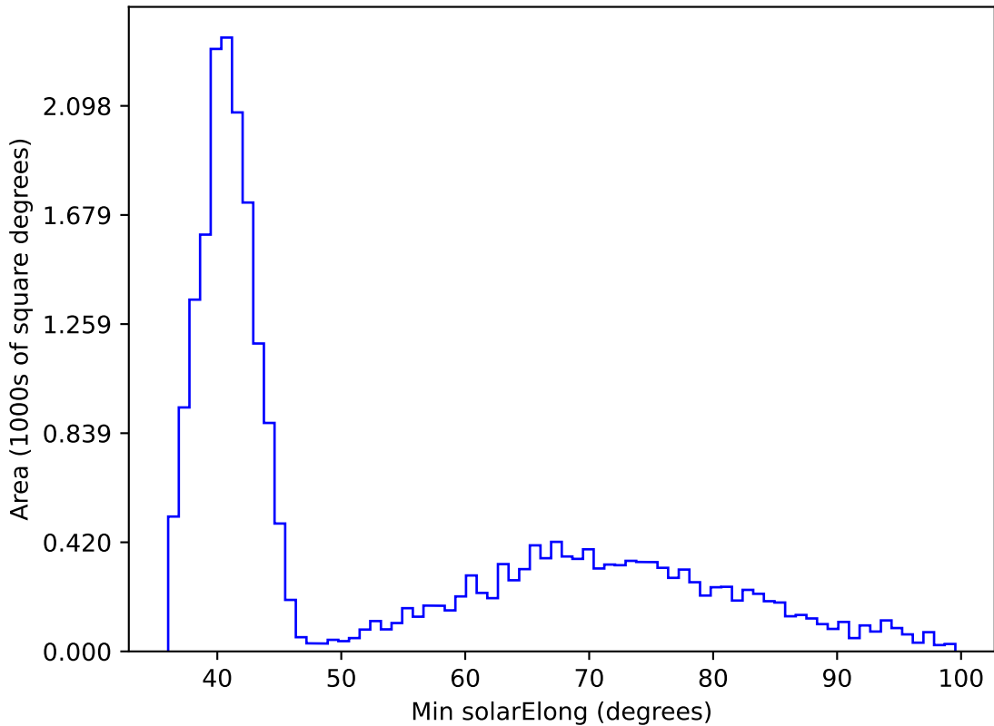
too_5_1v3.4_10yrs All sky i band: Min solarElong
