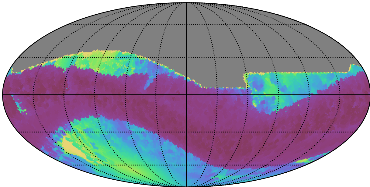
too_5_1v3.4_10yrs All sky all bands: Min solarElong
