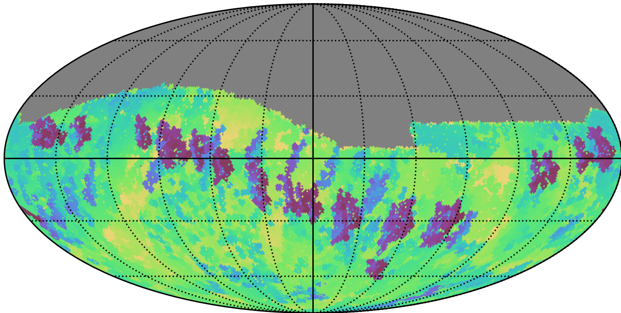
too_5_1v3.4_10yrs Yr 1 z band: Min skyBrightness
