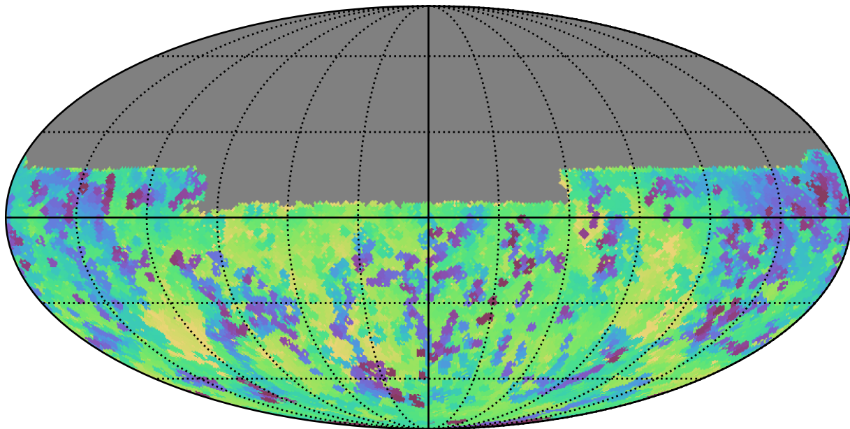
too_5_1v3.4_10yrs Yr 1 y band: Min skyBrightness
