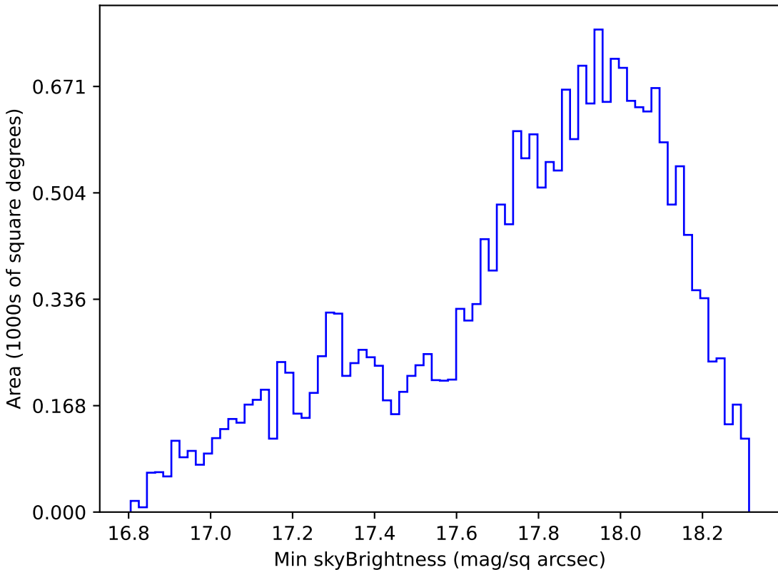
too_5_1v3.4_10yrs Yr 1 y band: Min skyBrightness
