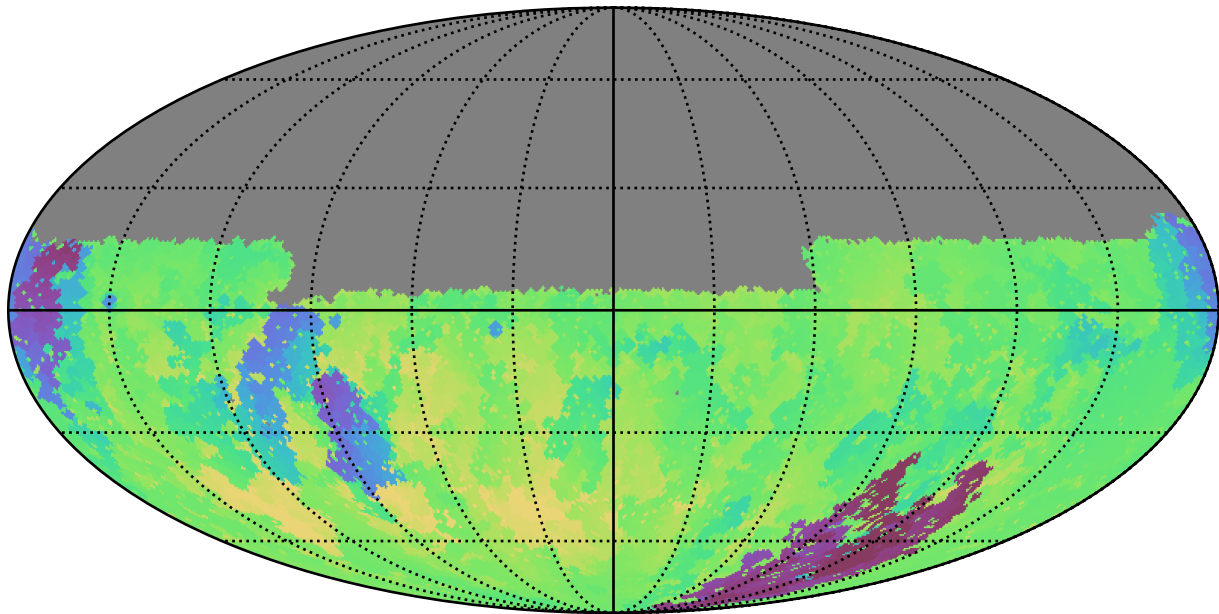
too_5_1v3.4_10yrs Yr 1 u band: Min skyBrightness
