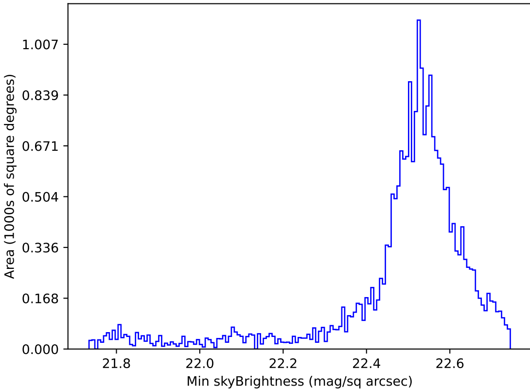
too_5_1v3.4_10yrs Yr 1 u band: Min skyBrightness
