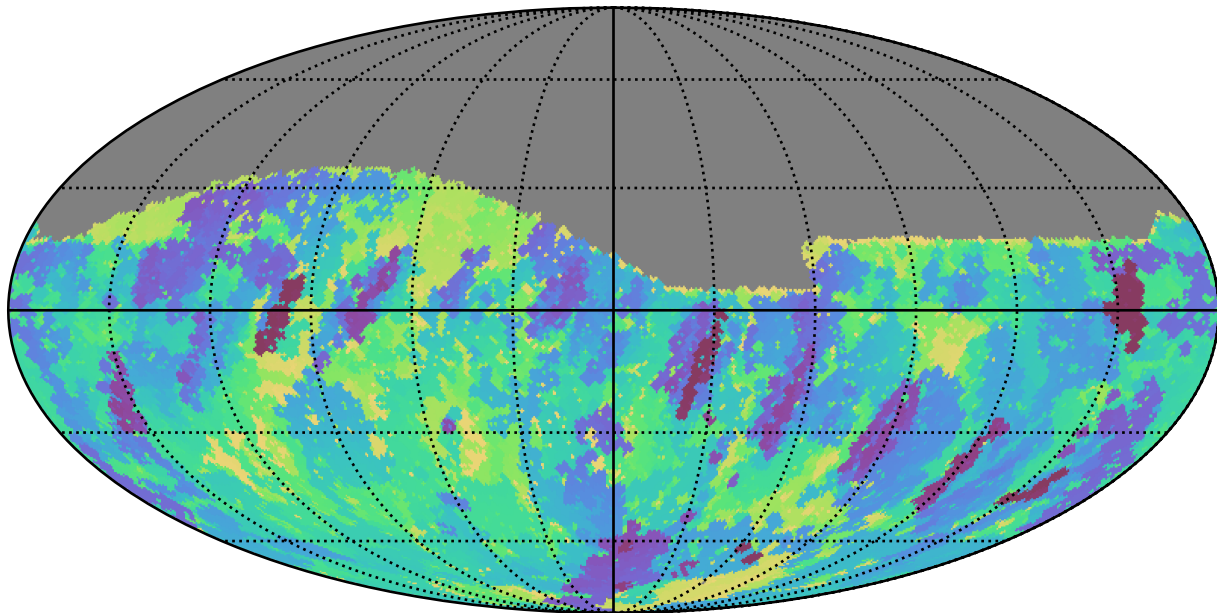
too_5_1v3.4_10yrs Yr 1 r band: Min skyBrightness
