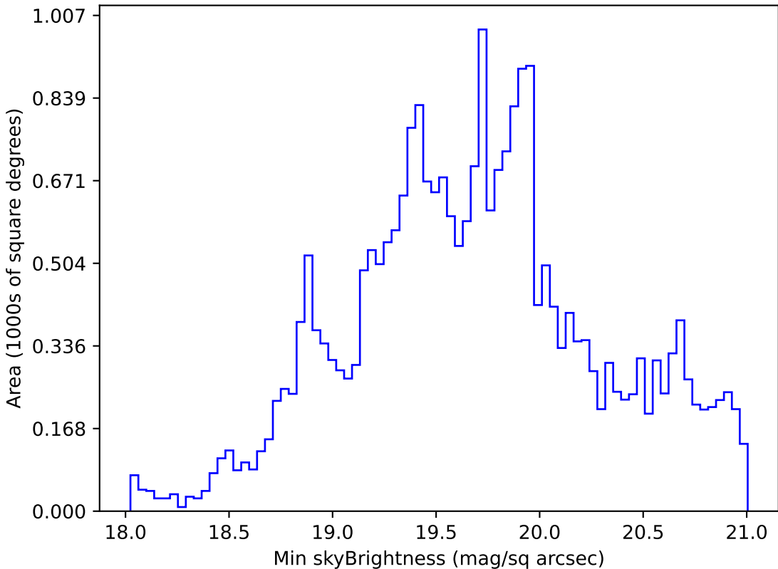
too_5_1v3.4_10yrs Yr 1 r band: Min skyBrightness
