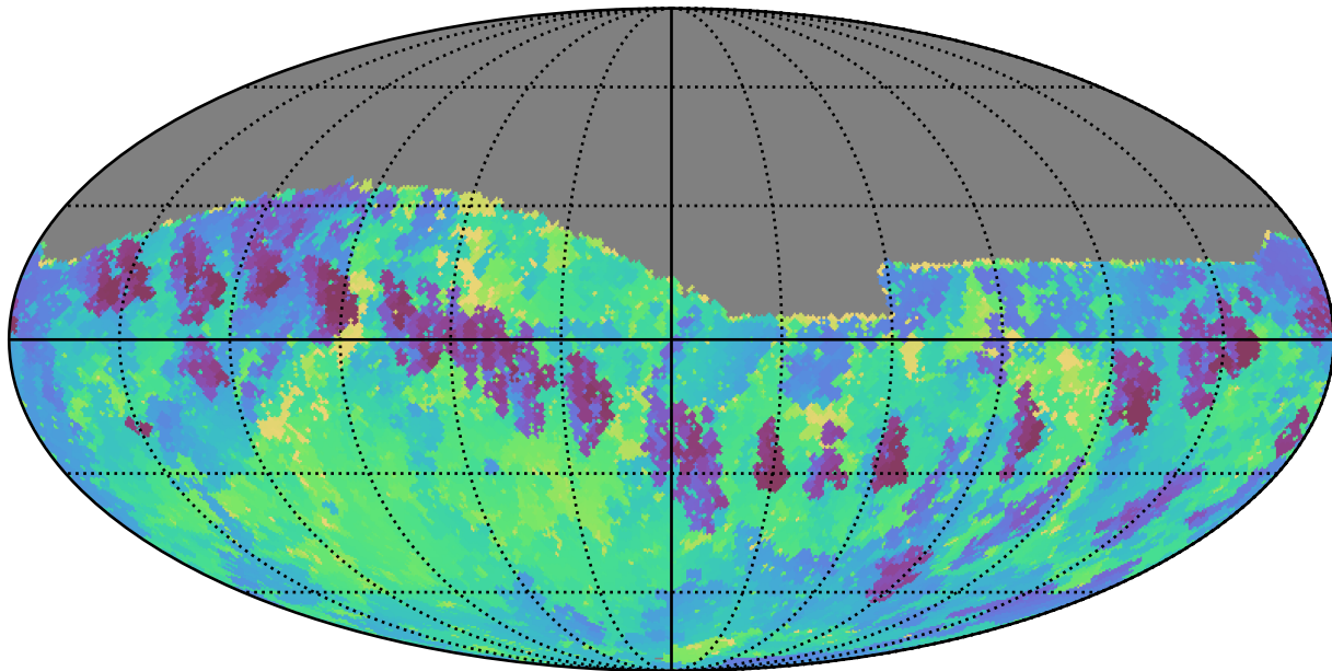
too_5_1v3.4_10yrs Yr 1 i band: Min skyBrightness
