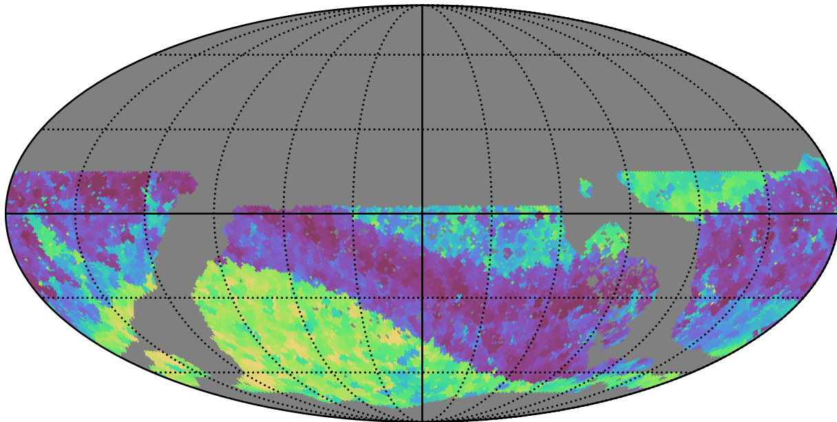
too_5_1v3.4_10yrs WFD z band: Min skyBrightness
