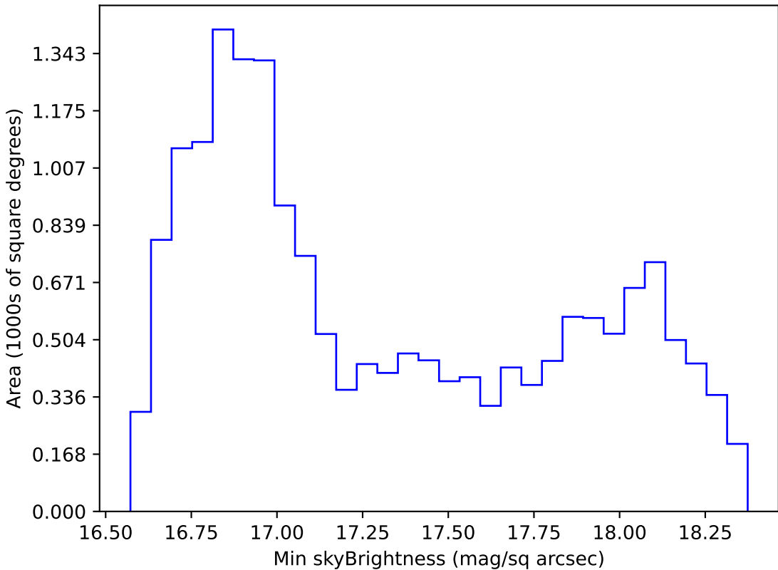
too_5_1v3.4_10yrs WFD z band: Min skyBrightness
