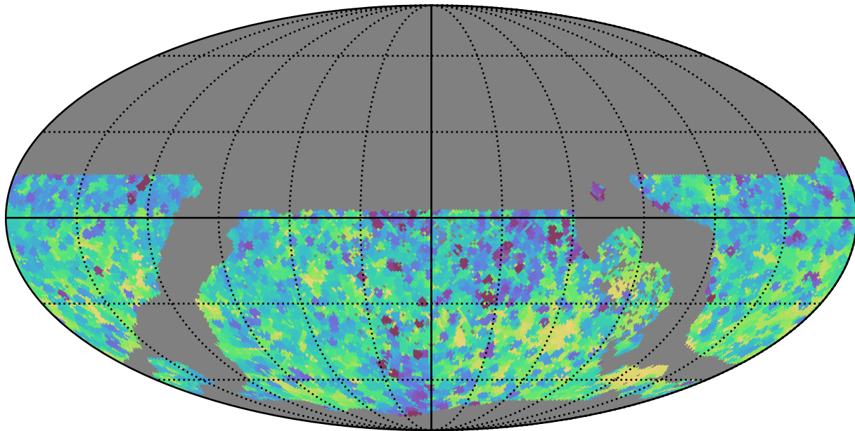
too_5_1v3.4_10yrs WFD y band: Min skyBrightness
