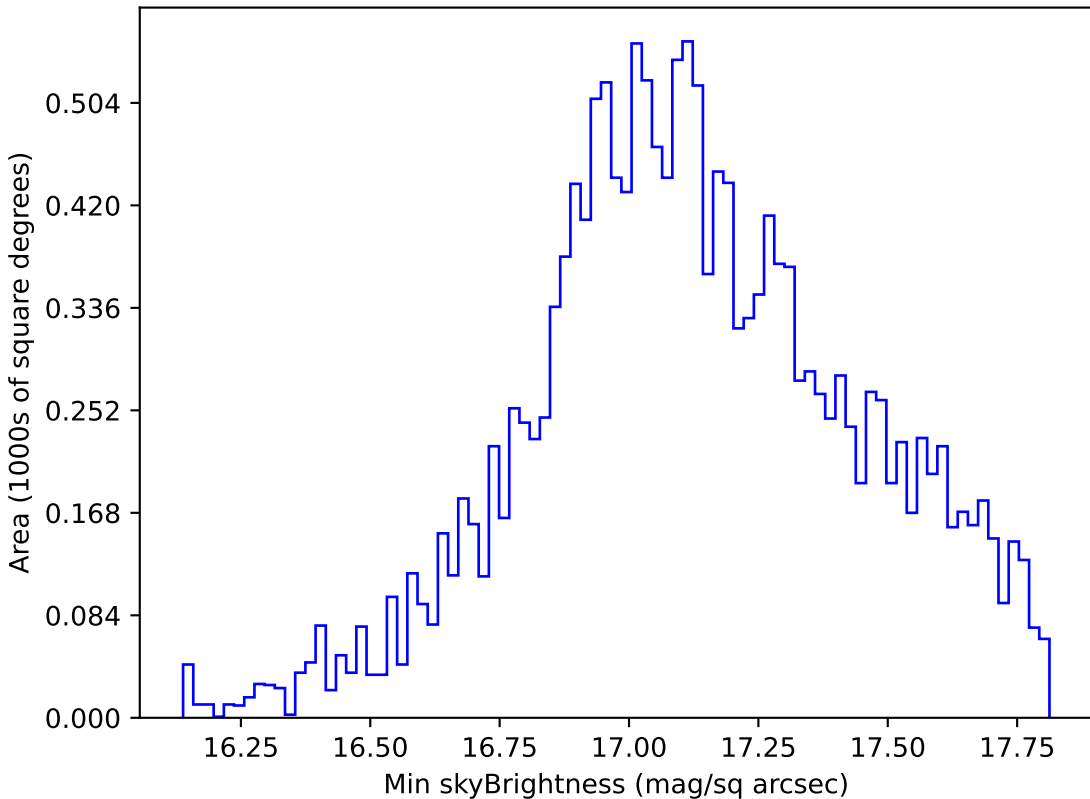
too_5_1v3.4_10yrs WFD y band: Min skyBrightness
